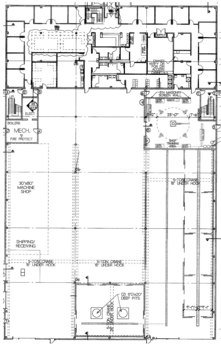
MAIN FLOOR
